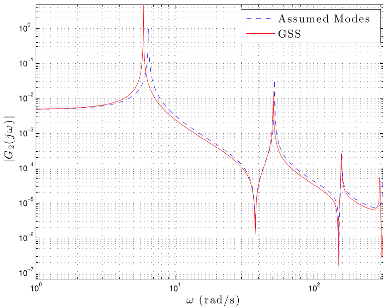
Fig. 9 Frequency response comparison tip mass model at beam midpoint, x = L/2 , using \phi_i(x)
